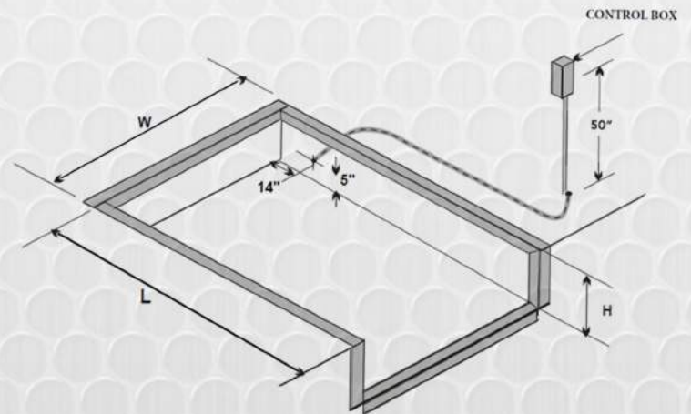
PIT DIMENSIONS
